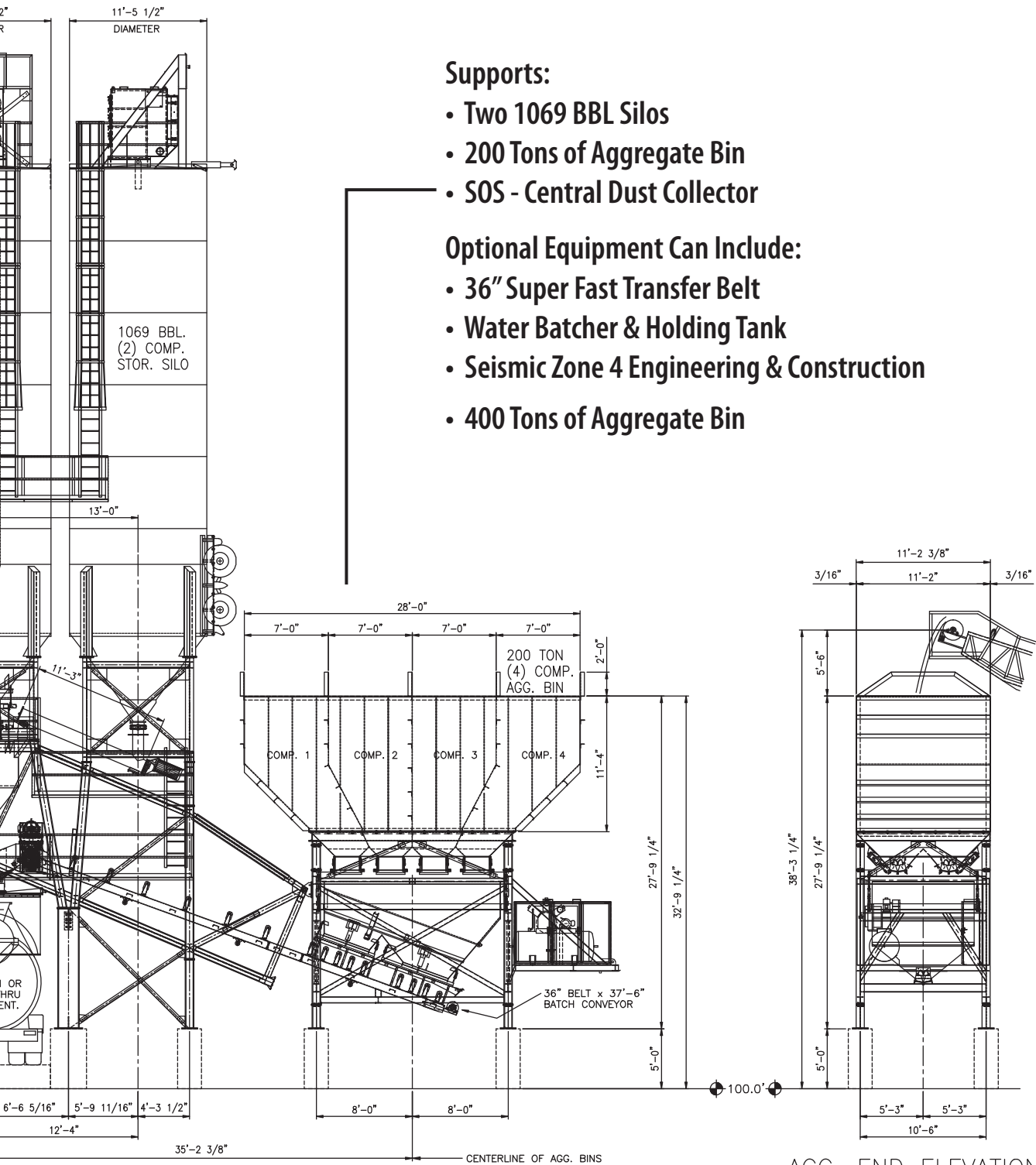
BATCH PLANT SIDE ELEVATION – OPERATING POSITION
